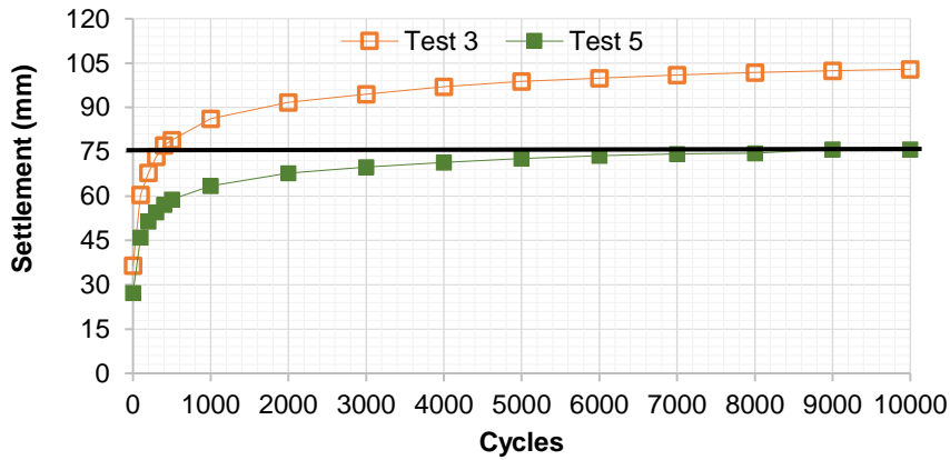
Figure 4: The settlement evolution with cycles at the base course surface centre for H=22cm.
