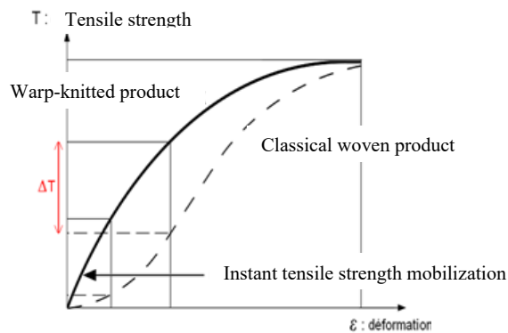
Figure 8. Tensile strength/elongation curve.
