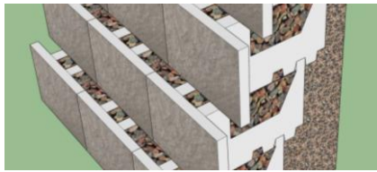
Figure 6. Ballast fill material.
