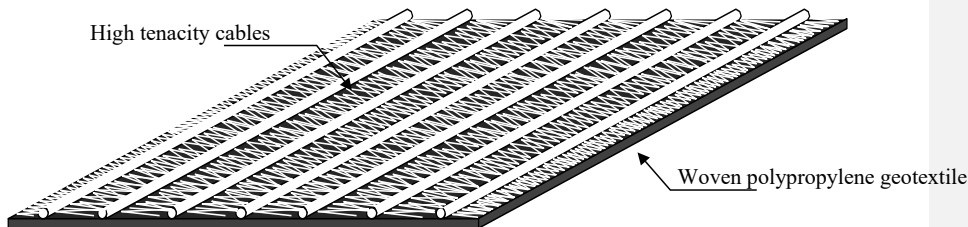
Figure 7. Structure of the geocomposite.
